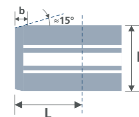
Diagram 6.03
