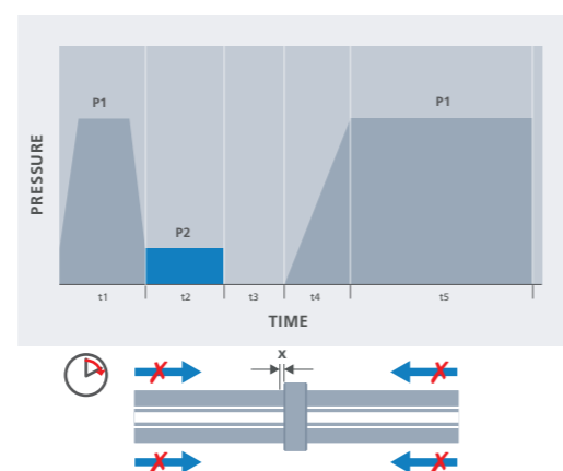
Diagram 6.10 – t2 Heating
