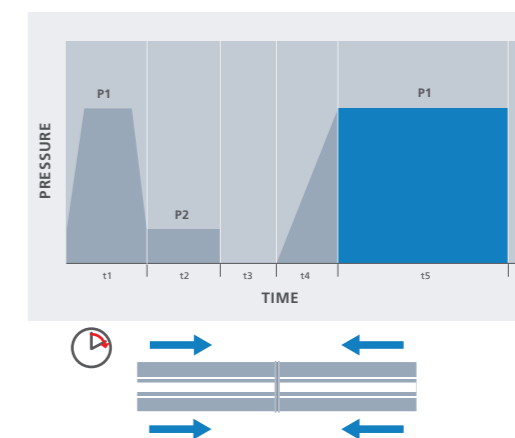
Diagram 6.13 – t5 Cooling
